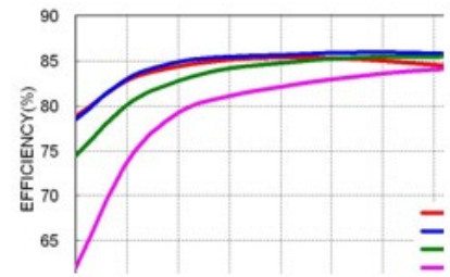
43MOP10-48S05WA Efficiency vs. Output Load
