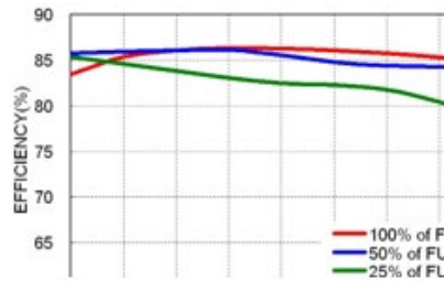
43MOP10-48S05WA Efficiency vs. Input Voltage
